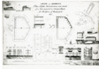
Plan of Fort Pulaski
